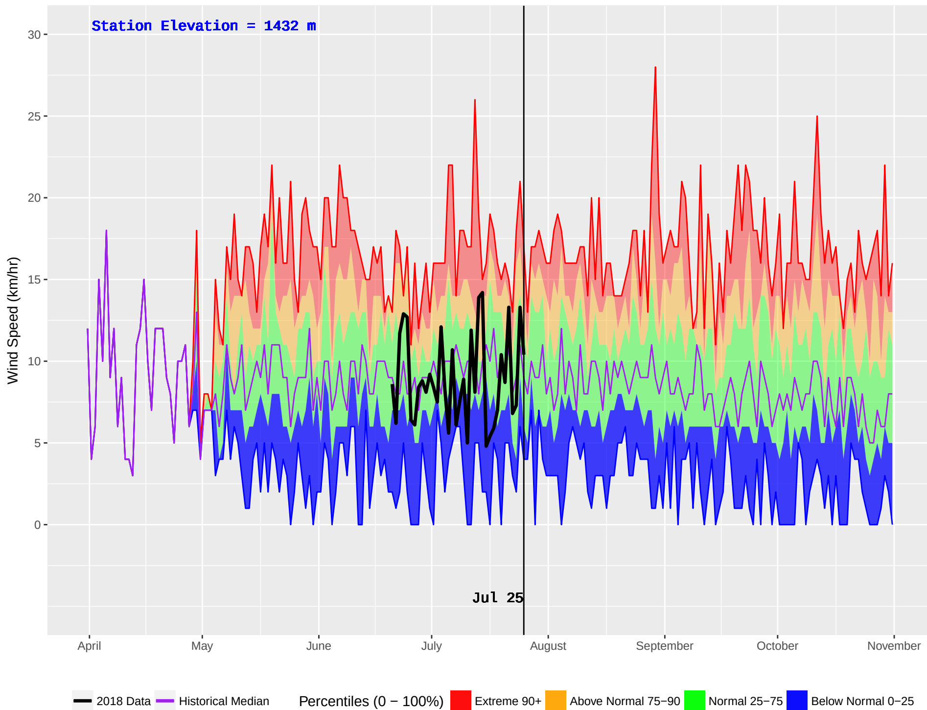
OCTOPUS CREEK (396) : Historical (2000–2016) and Current (2018) Noon Wind Speed
