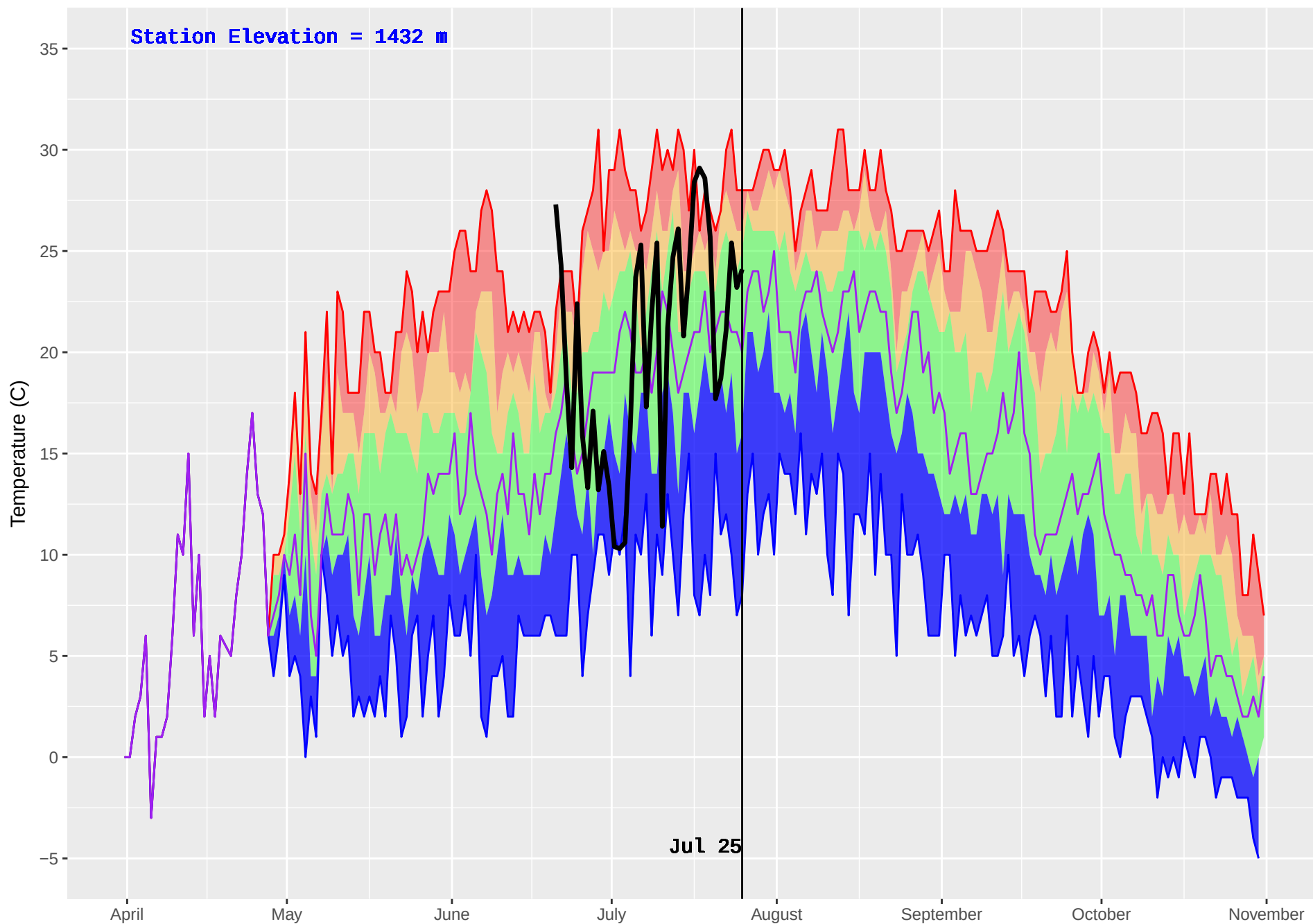
OCTOPUS CREEK (396) : Historical (2000–2016) and Current (2018) Noon Temperature
